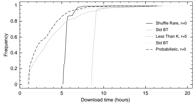
Fig. 3. Interesting experiments: CDF of peer download time
