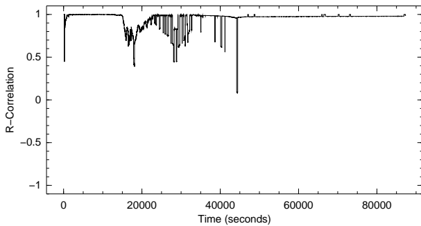
Fig. 6. Accuracy of block diversity estimate, probabilistic , r = 0
