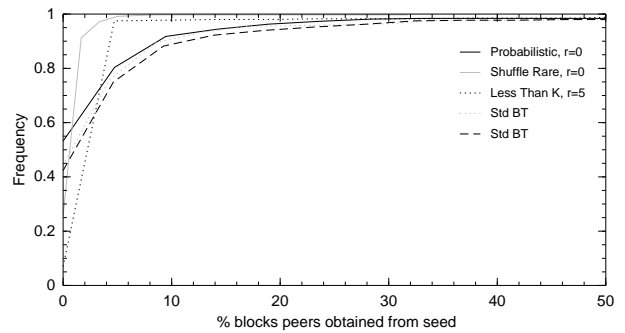
Fig. 2. Interesting experiments: CDF of source dependence
