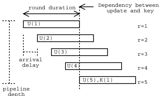
Figure 2: Pipelining rounds in NEO.
